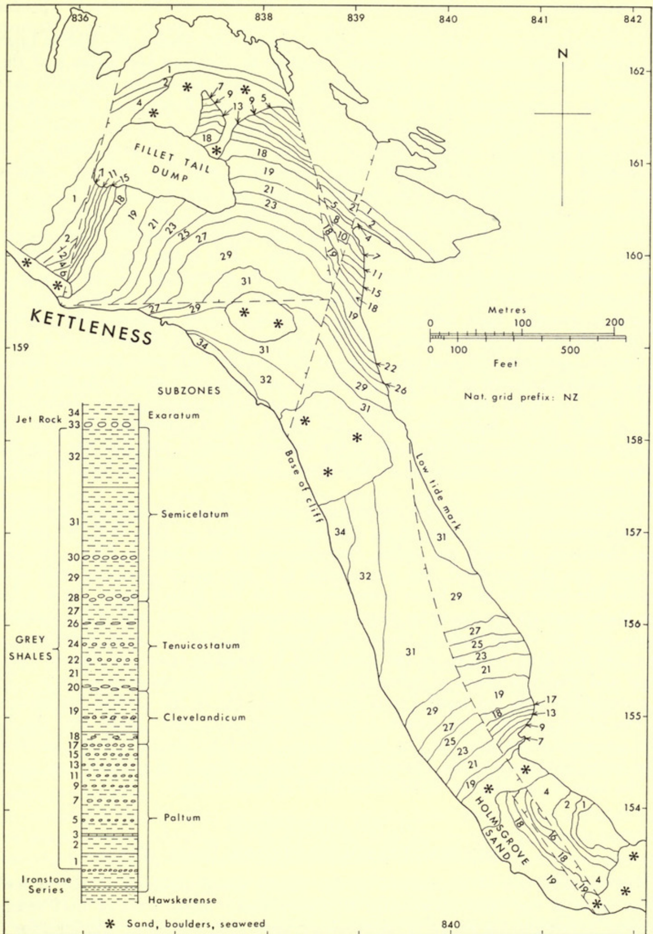
FIG. 3. Geological map of the Grey Shales on the foreshore at Kettleness.
