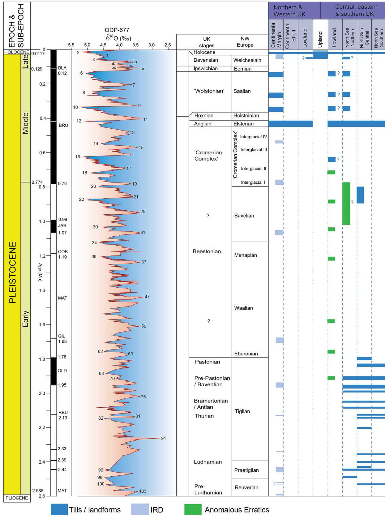
Fig. 1. The Quaternary timescale showing the marine isotope record (based on Lisiecki and Raymo, 2005) and projected temperate (pink) and cold (blue) stage intervals. Superimposed upon this timescale is evidence for the long-term glacial history of the UK utilising direct (e.g., tills, landforms) and
