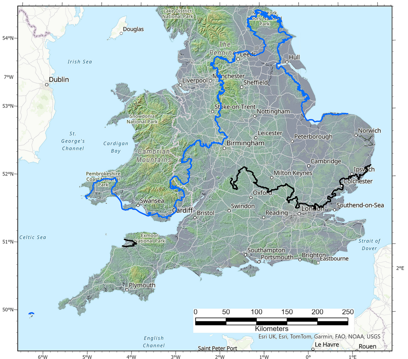
Fig. 7. Reconstructed limits of preserved evidence for both the Anglian (black line) and Late Devensian (blue line) glaciations. No differentiation is made here for uncertainty of the linework and readers are referred to Figures 8–11 for further information. Derived in part from DTM of Great Britain at 5 m resolution © Bluesky International Limited. Esri "World Topographic Map". Jan 4, 2024. Esri Sources: Esri, Ordnance Survey.
