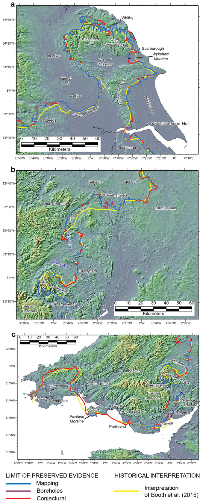
Fig. 11. Detailed maps of local areas of the limit of preserved evidence for the Late Devensian with local points of interest: (a) Eastern Sector – Yorkshire; (b) West Midlands and the Welsh Borders; (c) Welsh Borders and South Wales. Derived in part from DTM of Great Britain at 5 m resolution © Bluesky International Limited.
